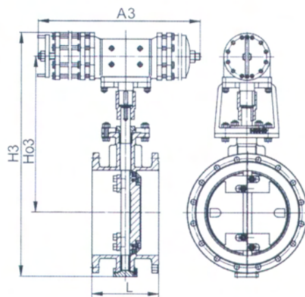
气动法兰连接蝶阀 Pneumatic Flanged Butterfly Valve
