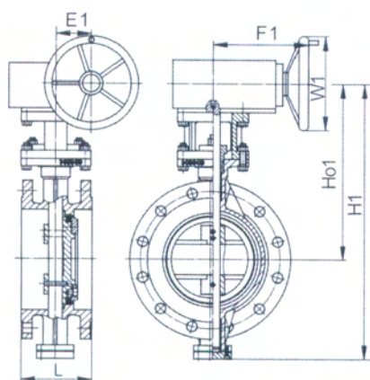
蜗轮蜗杆传动法兰连接蝶阀 Worm Gear Driven Flanged Butterfly Valve
