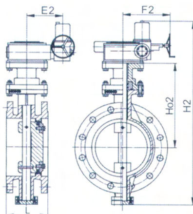
电动法兰连接蝶阀 Electric Flanged Butterfly Valve
